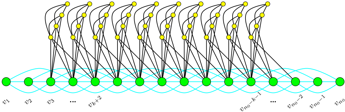
Figure 2: The graph G with k = 3 and d = 11 (and thus r = 1 ).
