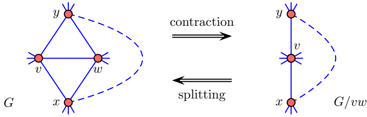
FIGURE 1. Contracting a reducible edge.
