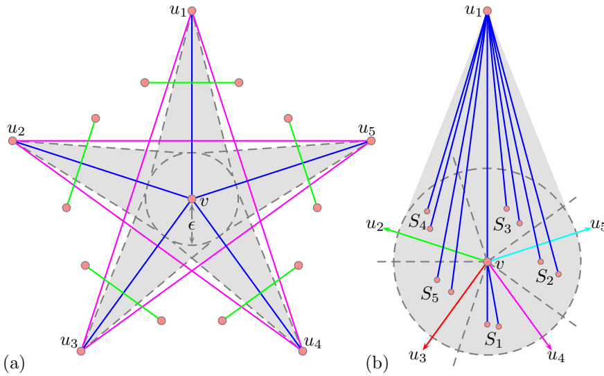
Fig. 4 (a) N_G(v) = \{u_1, u_2, \dots, u_5\} , T_\varepsilon(v) is shaded, and v is \varepsilon -empty. (b) The new edges coloured 1 in Proposition 5.
