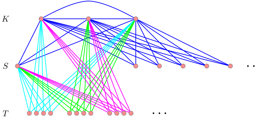
Fig. 8 The graph Q_k in Theorem 3 with k = 3 .
