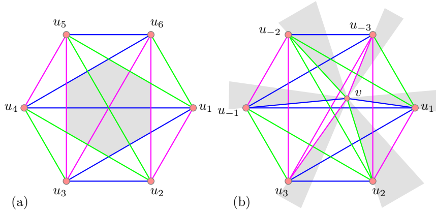
Fig. 6 (a) Book embedding of K_{2k} . (b) Geometric drawing of K_{2k+1} in which v is a fan.
