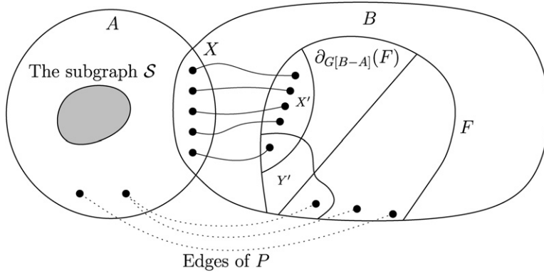
Fig. 1. An example of the separation (A, B) with the subgraphs S and F and possible sets X' and Y' .
