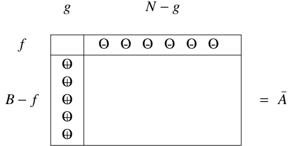
Figure 2.1 : An Optimal Dictionary ( \oplus = non-negative entry, \ominus = non-positive entry )
