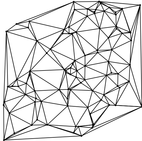
Figure 1: A minimum weight triangulation of 100 points
